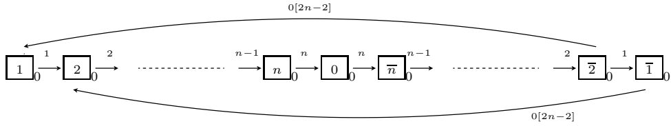
FIGURE 3. (Type B_n^{(1)} ) the crystal \mathcal{B}(\varpi_1)
