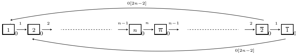
FIGURE 7. (Type A_{2n-1}^{(2)} ) the crystal \mathcal{B}(\varpi_1)
